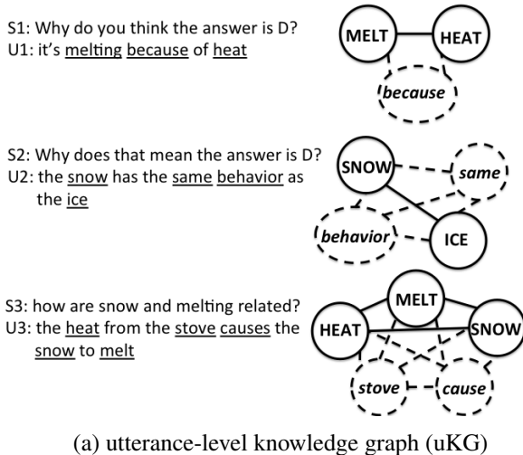
Figure 2: Every pair of concepts in each user utterance is related then aggressively pruned. (a) Utterance-level knowledge graphs represent individual utterances. Concepts (underlined, inset in nodes) are obtained by removing stopwords and stemming. An edge that either doesn't connect a question and support concept or else which connects concepts whose keywords in the user utterance have no intervening words ( intexts ) are pruned, indicated here with dashed lines. (b) The four remaining relations are stored in a dialog-level dKG.
